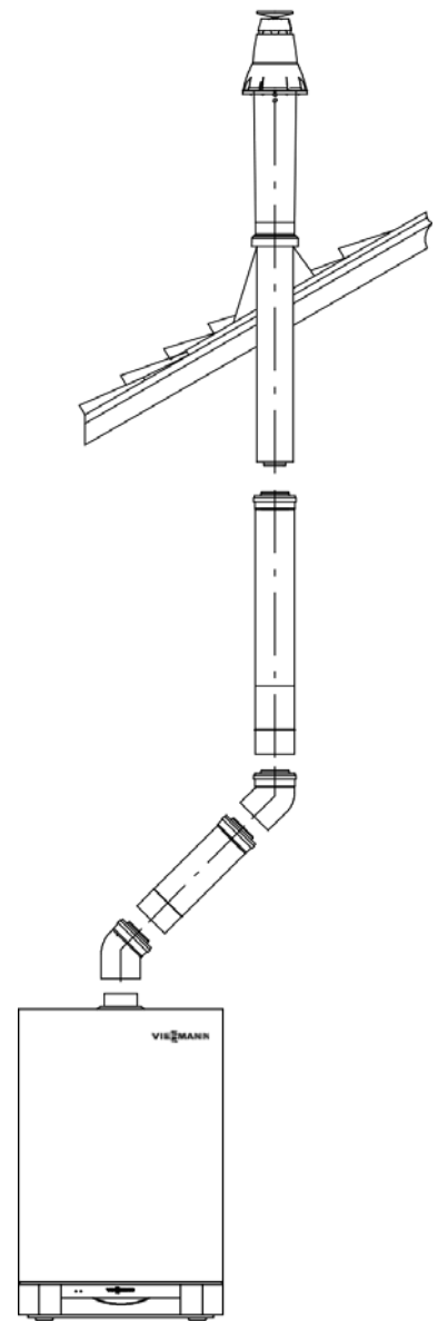
Sloped roof installation with offset
