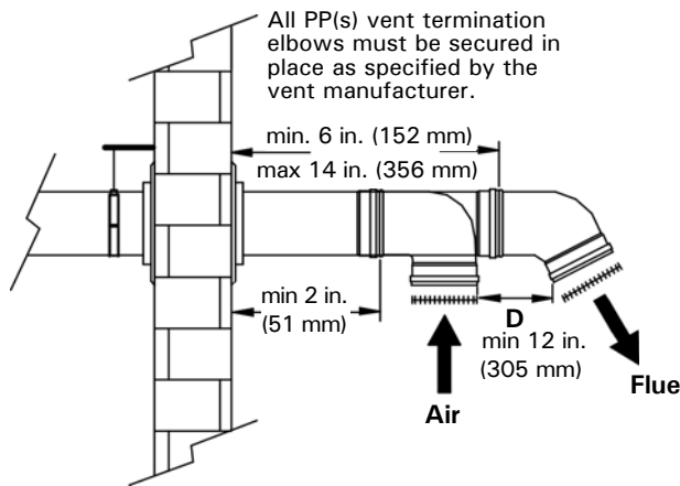
Side wall vent termination (side view)
